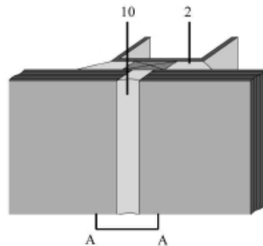
Figure 2B: A mullion detail.
